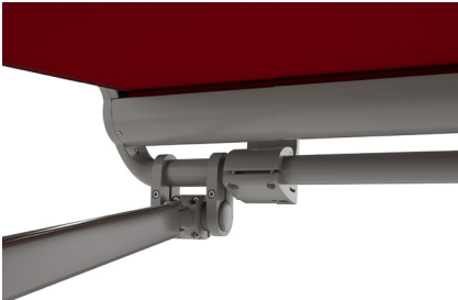
5) unique water drainage system and hidden cover pocket in the front profile
