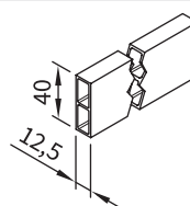
stand-off strip for wall sealing by the metre
