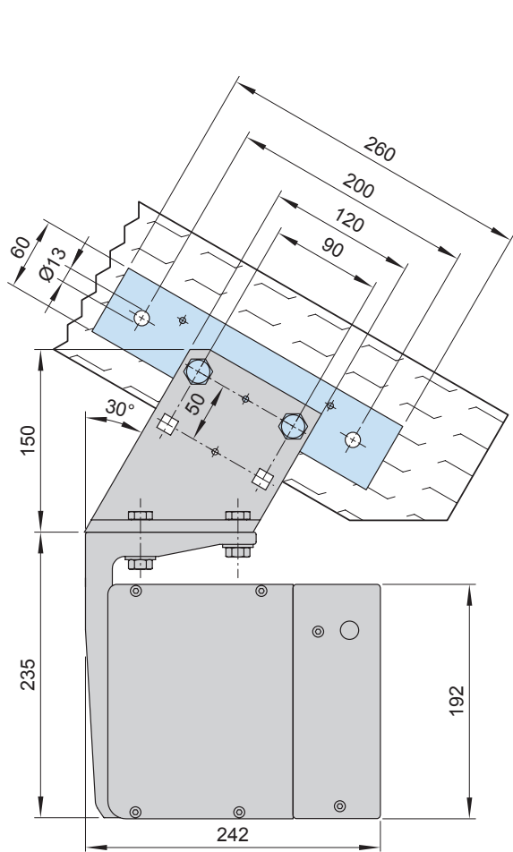
Eaves fixture bracket with backing plate for 75889.
