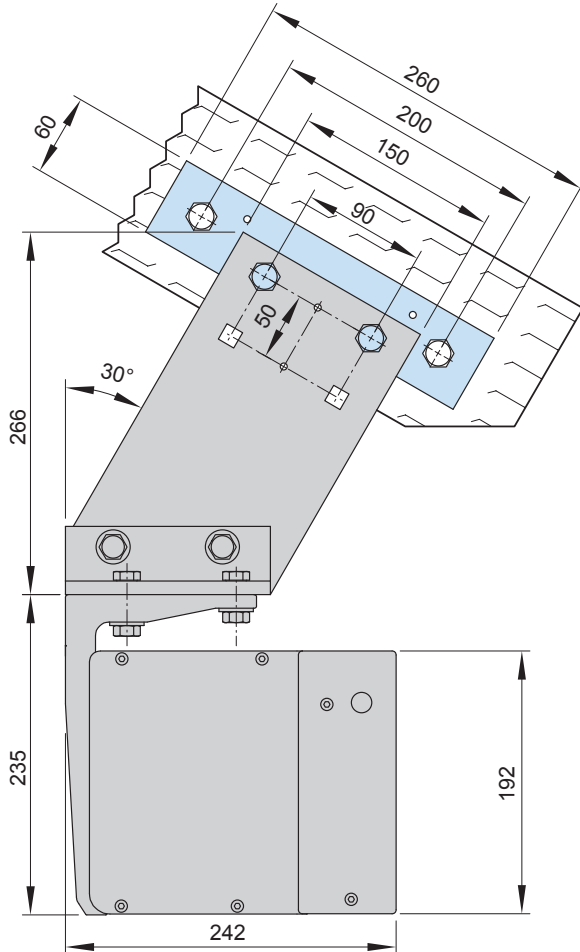
Eaves fixture bracket with backing plate for 71659.
