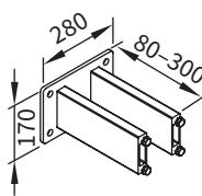
stand-off bracket 80-300 mm incl. insulating element
