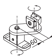
windmill track bracket 100 mm
