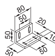
additional angled bracket for the bearing, gearbox and motor sides 50 × 50 × 80 mm fixture type 15
