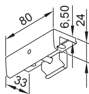
flat track bracket fixture type 10 and 15
