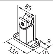
track bracket, with adjustable head 100 mm
