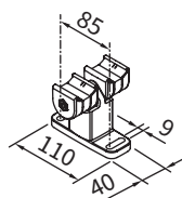
double track bracket with adjustable head 80 mm central bracket for 2 single units next to each other
