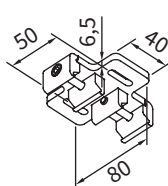
double track bracket plat 2 single units
