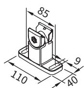
track bracket, with adjustable head 80 mm
