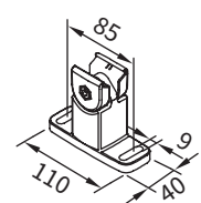
track bracket, with adjustable head 80 mm fixture type 20
