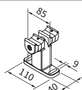
double track bracket with adjustable head 100 mm central bracket for 2 single units next to each other
