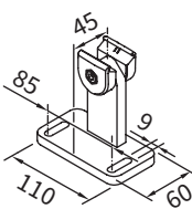
track bracket with offset footplate
