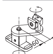
windmill track bracket 100 mm
