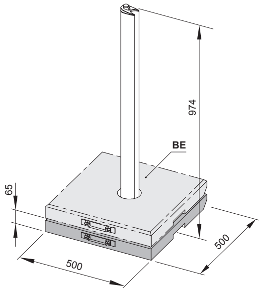
mobifix with additional granite slab to weigh it down
