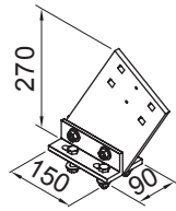
eaves fixture bracket 90 mm height of flat plate 270 mm
